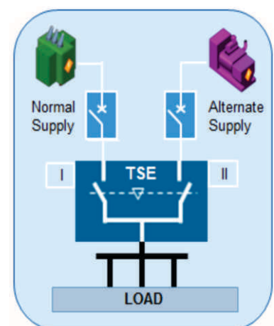
Fig.1 Basic outline of a TSE circuit
